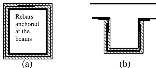
Figure C8.4: Indicative means of strengthening against diagonal compression: (a), closed-form strengthening, (b) open strengthening with strong end connection
