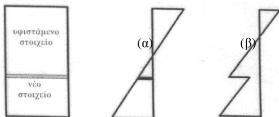
Fig. C8.1: Distribution of deformations within a composite section that is subjected to bending: (a) monolithic behaviour, (β) slip along the interface
