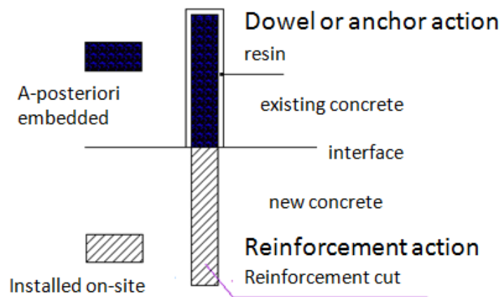
Figure C6.5: Rebar function during connection of new with existing concrete.
