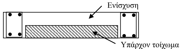
Figure C8.5: Indicative arrangement of a one-sided shear wall strengthening
