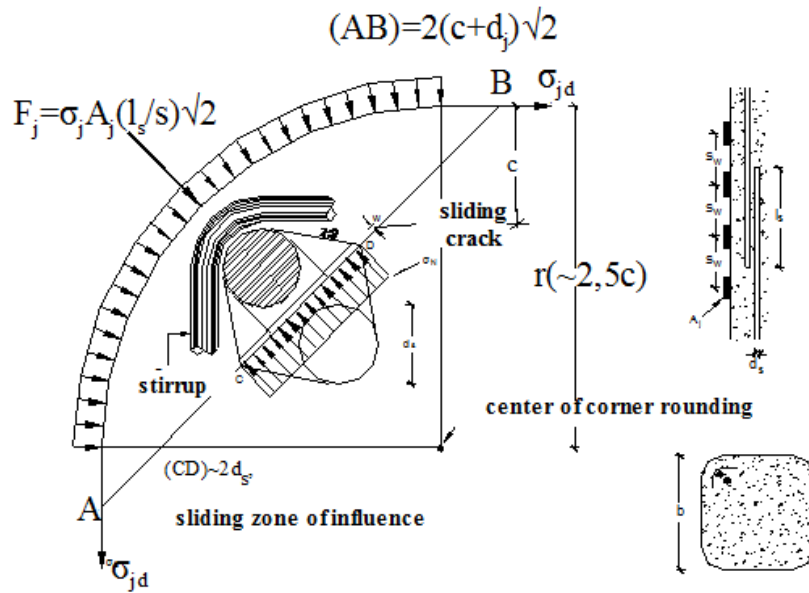
Figure C6.10: Activation of external confinement at the area of a corner, lapped rebar.
