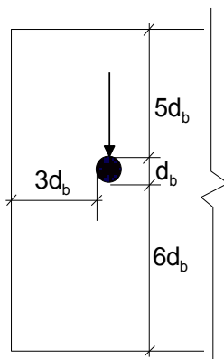
Figure C6.6: Definition of dowel cover
