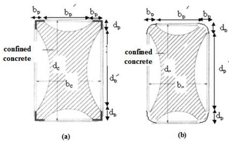
Figure C6.9 (a) Confinement using a steel cage (β) Confinement using FRPs – corner rounding, see § 4.4.3.e
