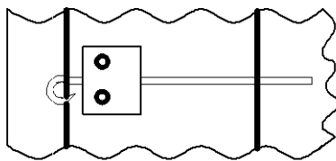
Figure C8.10: Indicative illustration of anchorage of horizontal reinforcement
