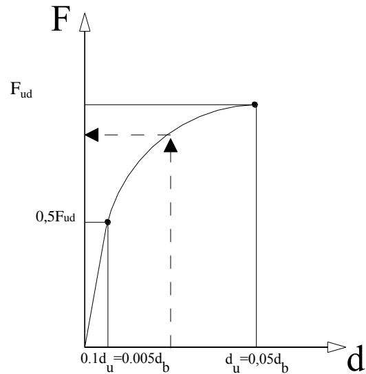
Figure C6.8: Constitutive law for the dowel behavior with sufficient concrete cover (also see eq. 6.10).
