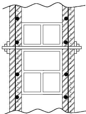
Fig. C8.10: Indicative cross section of the application of strengthening of an existing masonry infill.
