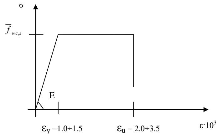
Stress-strain diagram of an equivalent diagonal strut for an unreinforced infill
