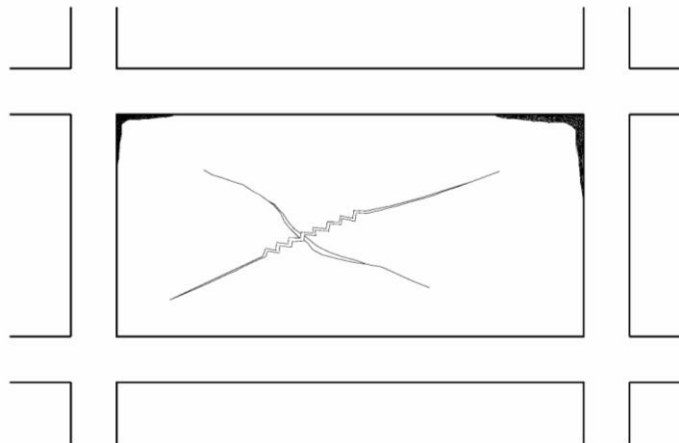
S2.2: Serious infill wall damage, cracks > 5mm
