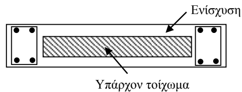
Figure C8.6: Indicative arrangement of a full-sided, closed jacket, shear wall strengthening
